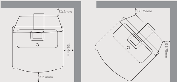
Standard Installation
